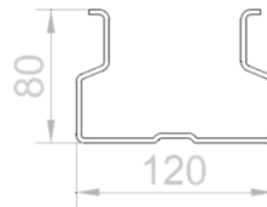
Figure 1. Upright Section and Dimensions.
