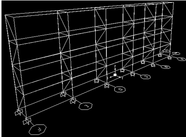
Figure 3. 3D View of the Model Configuration.
